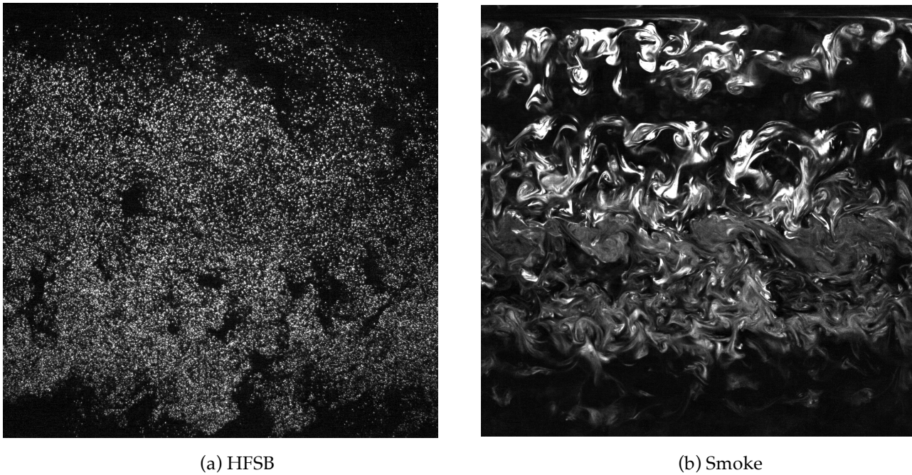
Fig. 6 1024x1024 snapshots of smoke seeding (b) and HFSB seeding (a) in the mixing layer.
