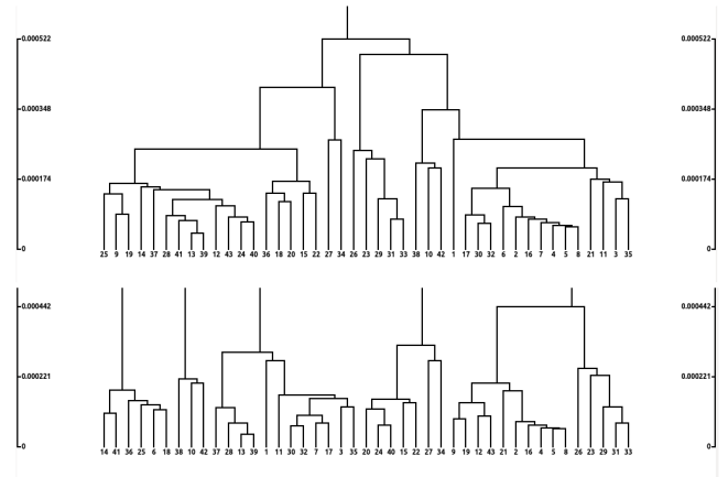
Fig. 5. Dendrograms obtained by agglomerative clustering on local speaker hypotheses, unconstrained (top); constrained (bottom)
