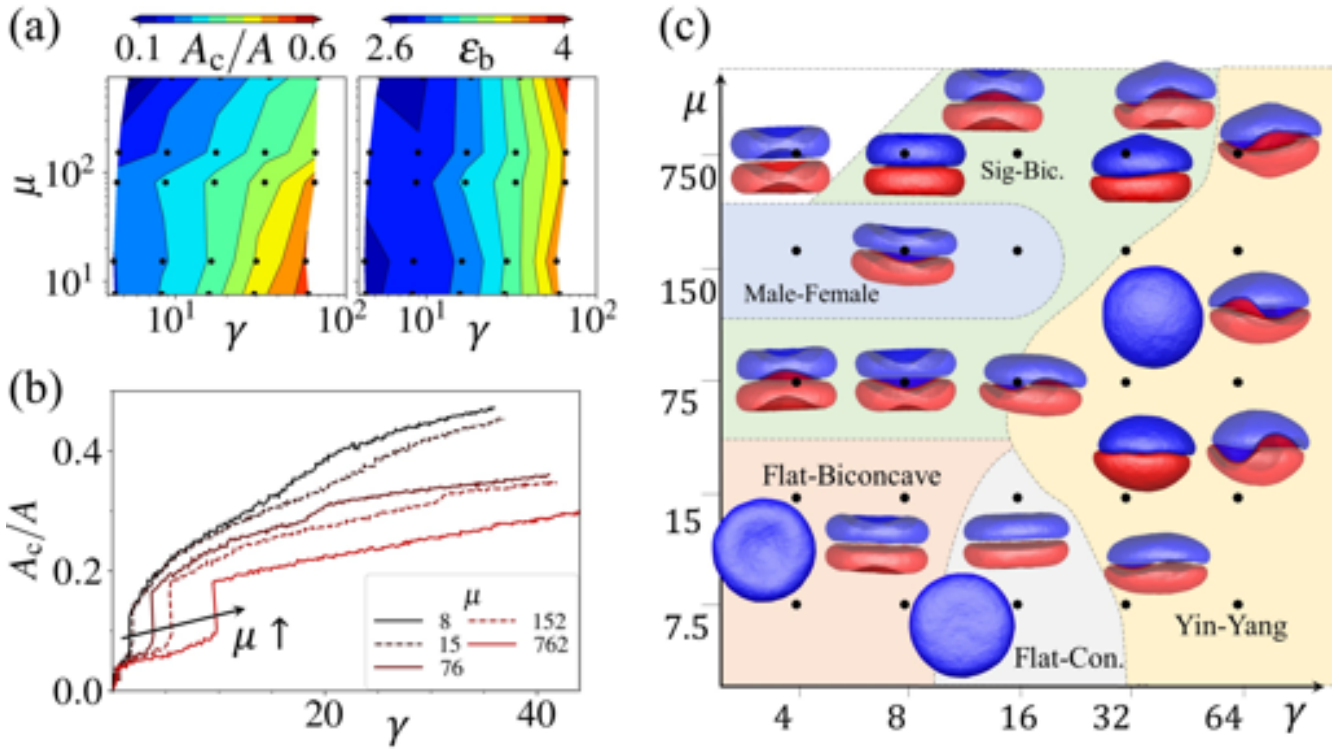
Fig. 7 RBC doublet configurations as a function of spectrin network's reduced shear modulus \mu = GA/8\pi\kappa_c and reduced adhesion strength \gamma at a constant reduced volume v = 0.64 . (a) Contour plots show the contact area and the reduced bending energy. The black dots ( \bullet ) represent the values for which simulations have been performed. (b) Dependence of the contact area on adhesion strength for different \mu values. Discontinuity in the contact area is observed when one or both RBCs loose their original biconcave shape. (c) Phase diagram of RBC doublets as a function of \gamma and \mu , where different phases are separated by various colors. The phase boundaries are drawn schematically to guide the eye. The side and section views of some configurations are shown, omitting some shapes for more clarity. The low shear moduli approximate vesicle doublets. The membrane is assumed to be stress-free in its biconcave shape with v = 0.64 .
