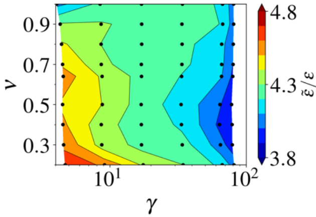
Fig. 4 The ratio of the effective adhesion energy \tilde{\epsilon} to the pairwise energy \epsilon . This ratio depends weakly on the configuration of the two adhered RBCs, as illustrated in Fig. 3. Simulations are conducted for the system until it reaches equilibrium. The reported data are averaged over 250 uncorrelated points in simulations from the equilibrium states. On average, \tilde{\epsilon}/\epsilon = 4.23 \pm 0.03 .
