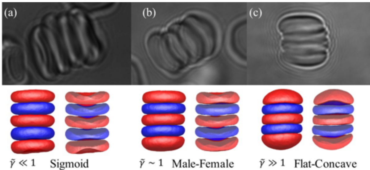
Fig. 11 Various rouleau phases in experiments and simulations. The doublet S-B and M-F phases impose no limit on the size of the rouleau. However, the F-C rouleaux are strongly dependent on the number of interacting RBCs and their reduced volumes. The nucleation point of a F-C rouleau is a Yin-Yang doublet.
