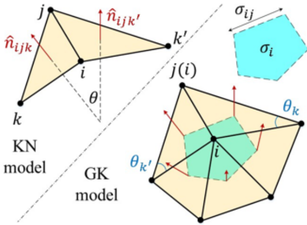
Fig. 1 Schematic of the two discretization models for the bending energy. The KN discretization 35 in Eq. (2) considers the bending between each two triangles, while the GK discretization 32 in Eq. (3) represents the bending of each vertex with respect to all of its linked vertices.
