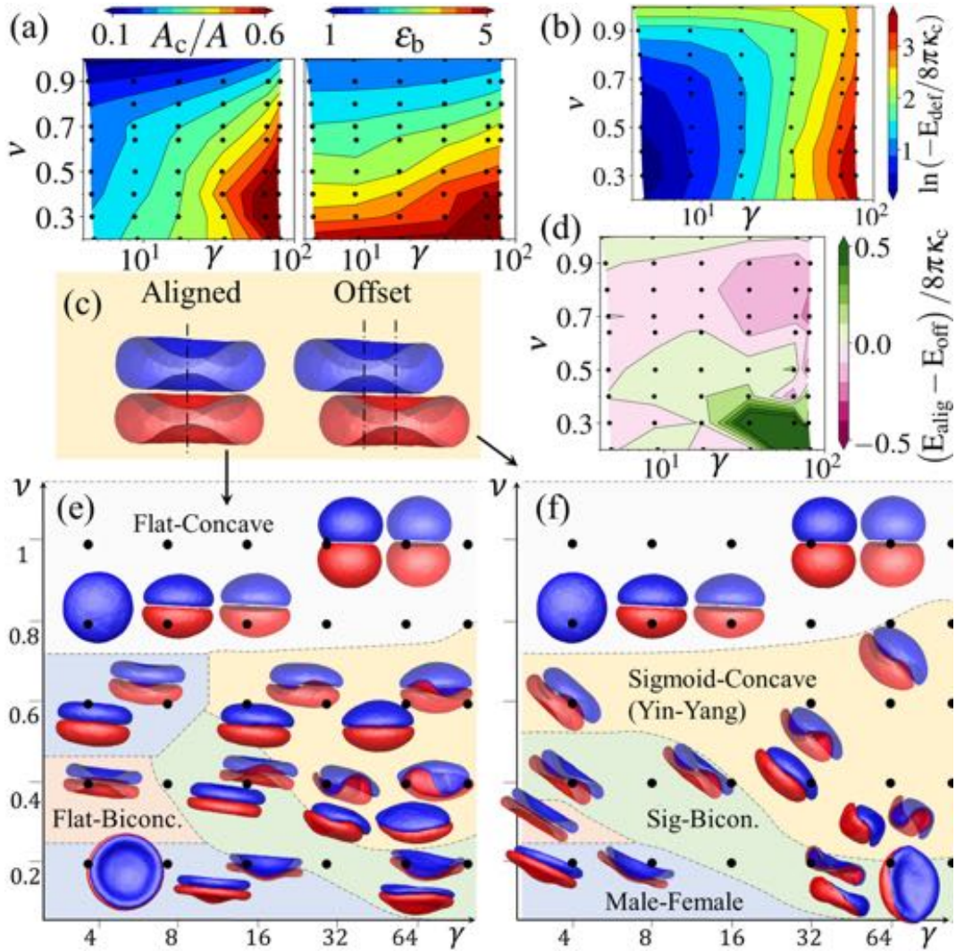
Fig. 5 RBC doublet configurations as a function of v_1 = v_2 = v and \gamma with aligned and offset first point of contact. (a) Contour plots for the contact area and the reduced bending energy for the aligned RBCs. (b) Contour plot for the difference between the free energy of the doublet and the free RBCs (deformation energy). The change in free energy is normalized by the bending energy of a vesicle with bending modulus \kappa_c , 8\pi\kappa_c , and the colorbar has a logarithmic scale. The black dots ( \bullet ) in contour plots represent the values for which simulations have been conducted. (c) The configuration of a doublet depends on the way the RBCs make their first contact. RBCs can make the first contact while they are in aligned or offset configurations. (d) The difference between the free energy of the doublets in the aligned and offset cases. If E_{\text{alig}} - E_{\text{off}} is positive, it means that the offset doublet has a smaller free energy, so that it is a more favorable configuration. The phase diagrams of the (e) aligned and (f) offset cases are different in the region, where E_{\text{alig}} - E_{\text{off}} is positive. Various phases are distinguished by their cross-sectional views. The black dots ( \bullet ) in the phase diagrams represent performed simulations. Note that the phase boundaries are drawn schematically to guide the eye.
