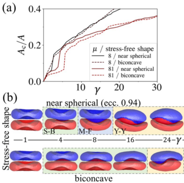
Fig. 8 Effect of stress-free shape of RBCs on doublet phases for v_1 = v_2 = 0.64 . (a) Contact area as a function of \gamma for biconcave and near spherical (with eccentricity 0.94) stress-free shapes. (b) The shapes of RBC doublets for \mu = 81 , showing appreciable differences for the two stress-free shapes. The boundaries between different shapes are drawn schematically to guide the eye.
