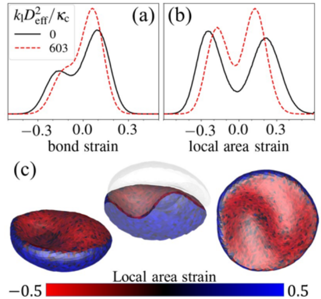
Fig. 9 Effect of the local area constraint in the membrane model on a Yin-Yang doublet for \gamma \approx 85 , \mu = 80 , and v_1 = v_2 = 0.64 . (a) Bond strain distributions from simulations with and without local area constraint. The bond strain is defined as l/l_0 - 1 , where l is the length of a deformed bond and l_0 is its corresponding equilibrium length. (b) Distributions of local triangular area strains. The area strain is defined as A/A_0 - 1 , where A is the area of a deformed triangle in the spring network and A_0 is its imposed area at biconcave equilibrium shape. (c) Distribution of local area strains on RBCs within a Yin-Yang doublet. The RBC membranes show a compressive deformation (or negative area strains) at the contact area and are stretched primarily at the free surfaces characterized by positive area strains.
