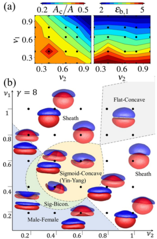
Fig. 6 RBC doublet configurations as a function of v_1 and v_2 at a constant adhesion strength \gamma = 8 . (a) Contour plots show the contact area and the reduced bending energy of the first RBC as a function of v_1 and v_2 . The black dots (•) represent the values for which simulations have been performed. (b) The side and section views of some configurations are shown in the phase diagram, omitting some shapes for more clarity. The different phases are separated by different colors. The S-B phase occurs in a narrow region between Yin-Yang and M-F phases. The membrane is assumed to be stress-free in its biconcave shape with v = 0.64 . The phase boundaries are drawn schematically to guide the eye.
