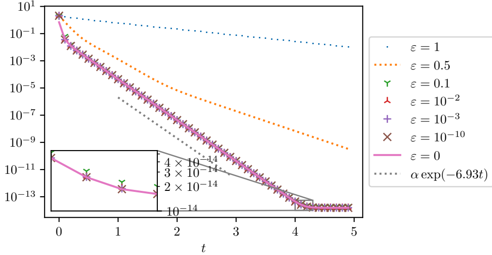
FIGURE 8. Test 3. Comparison of the rate of convergence of \|f^\varepsilon - m_f \mathcal{M}\|_{2,\gamma} for different values of \varepsilon , in the Fokker-Planck case.
