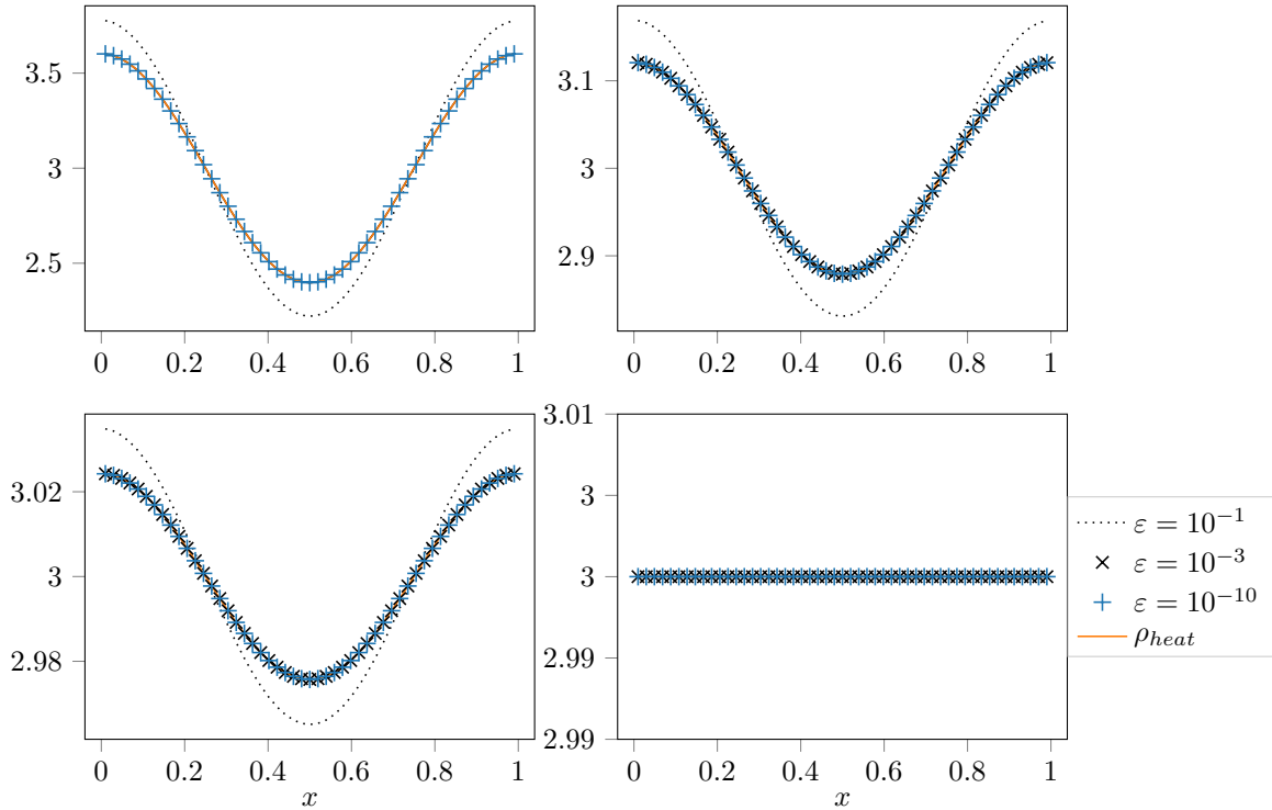
FIGURE 3. Test 1. Comparison of the solution to the heat equation obtained from the scheme (3.23) (solid line) with the solution obtained with the Fokker-Planck scheme (4.5) with different \varepsilon , at times t = 0.1, 0.2, 0.3 and 10 .
