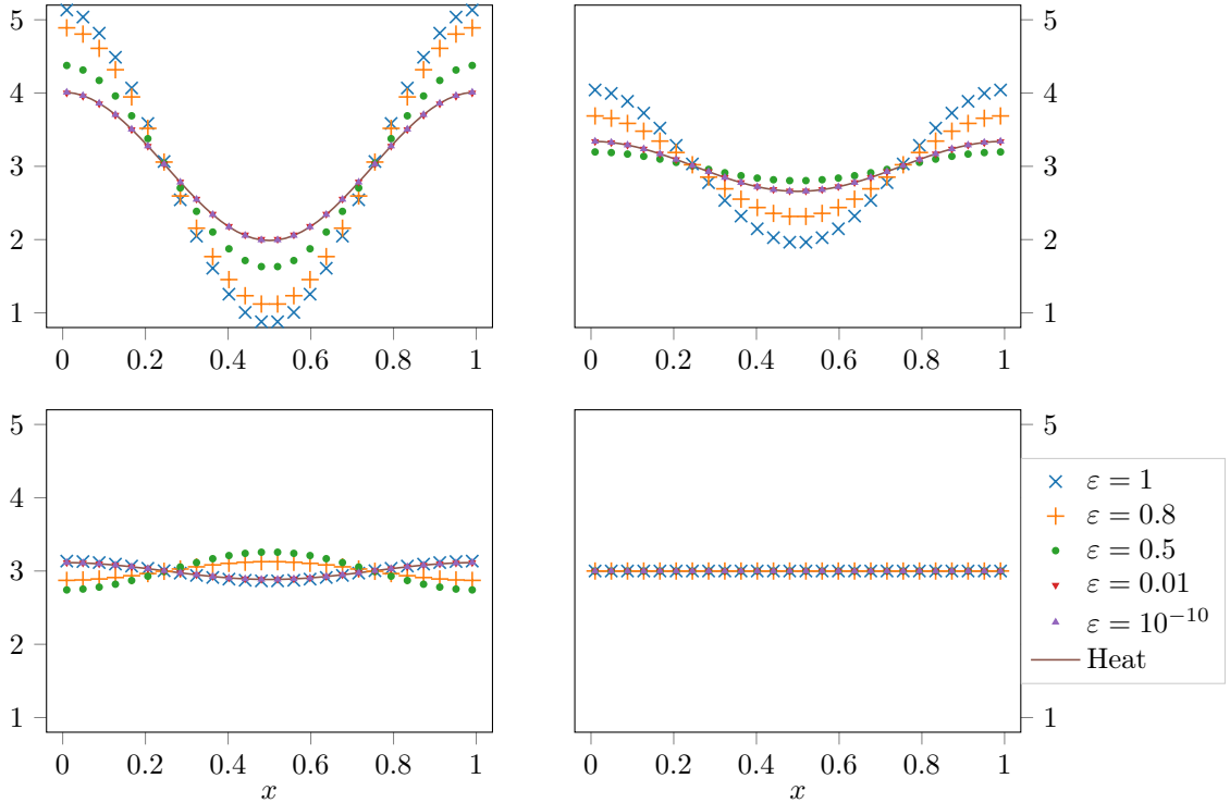
FIGURE 4. Test 1. Comparison of the solution to the heat equation obtained from the scheme (3.23) (solid line) with the solution obtained with the BGK scheme (4.6) with different \varepsilon , at times t = 0.05, 0.1, 0.15 and 10 .
