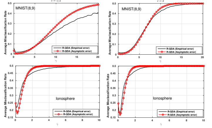
Figure 2: Performance of the R-QDA classifier applied to both data sets given by Table I in terms of the average classification error for different values of the ratio c . The first row gives the performance of the R-QDA classifier when applied to MNIST data set whereas the second row gives its performance when applied to the Ionosphere data set. The x-axis is the regularization parameter \gamma . In both data sets, we consider equal training, i.e. n_0 = n_1 .
