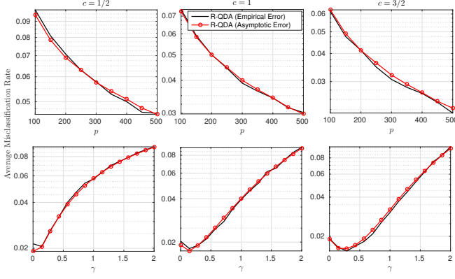
Figure 1: Performance in terms of the testing classification error of the regularized QDA classifier with equal training, n_0 = n_1 . The x-axis in the first row is the number of features p for \gamma = 1 while in the second row is the regularization parameter \gamma for p = 300 features.
