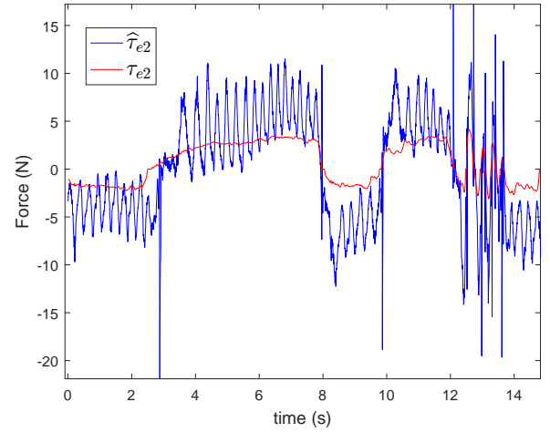
Fig. 8: Force measured by the sensor \tau_{e2} in red and estimated force \hat{\tau}_{e2} in blue
