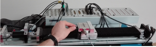
Fig. 7: Co-manipulation experiments, the operator apply a specific force on the force sensor of the robot presented into Fig. 1.
