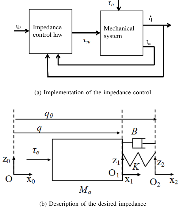
Fig. 11: Definition of the impedance control law
