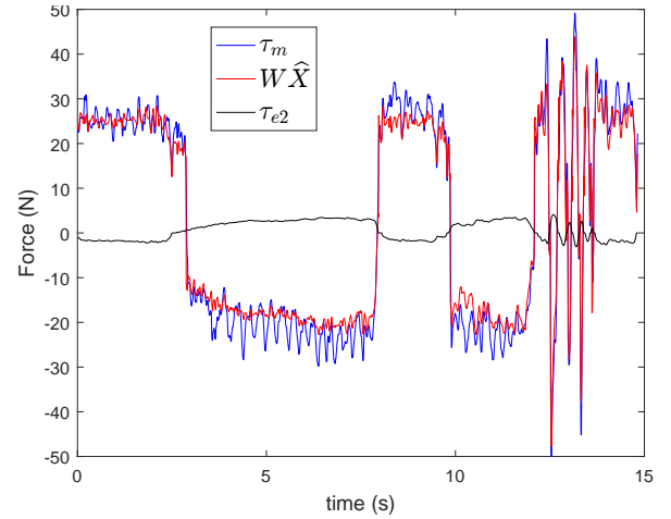
Fig. 10: Force applied by the motor \tau_m in blue, and estimated force W\hat{X} in red and effort from the operator \tau_e in black.
