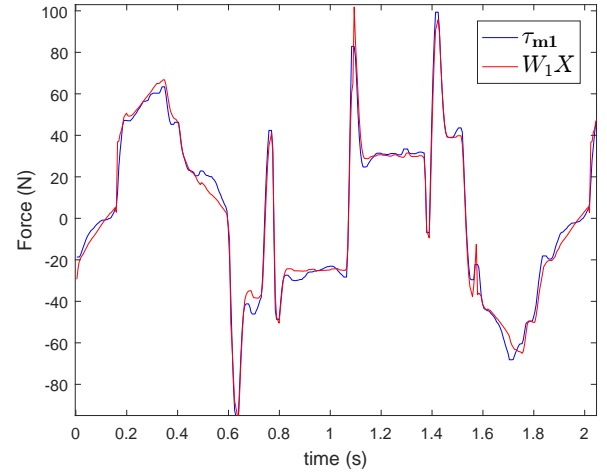
Fig. 6: Force from the motor \tau_{m1} in blue and \mathbf{W}_1\mathbf{X}_1 in red.
