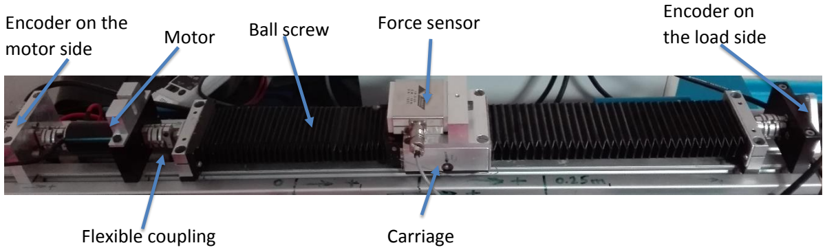
Fig. 1: Components of the EMPS robot.
