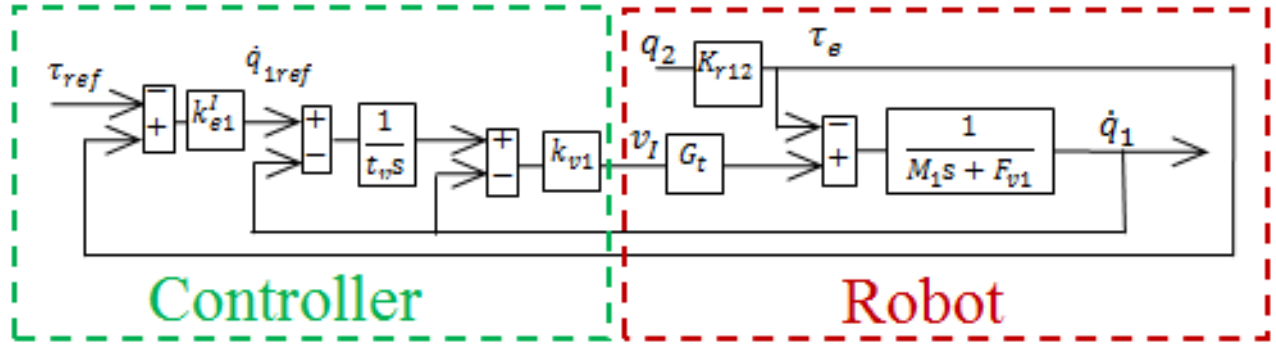
Fig. 4: Cascaded closed loop of speed and force in the case of co-manipulation.
