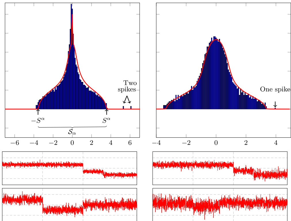
Figure 2: Two graphs generated upon the DCSBM with K = 3 , n = 2000 , c_1 = 0.3 , c_2 = 0.3 , c_3 = 0.4 , \mu = \frac{1}{2}\delta_{q(1)} + \frac{1}{2}\delta_{q(2)} , q(1) = 0.4 , q(2) = 0.9 and two different affinity matrices \mathbf{M} . (Left) M_{ii} = 12 , M_{ij} = -4, i \neq j , (Right) : M_{ii} = -3 , M_{ij} = -10, i \neq j , (Top) : Eigenvalue distribution of \mathbf{L}_\alpha , \alpha = 0 . (Bottom) : First and second leading eigenvectors of \mathbf{L}_\alpha , \alpha = 0 .
