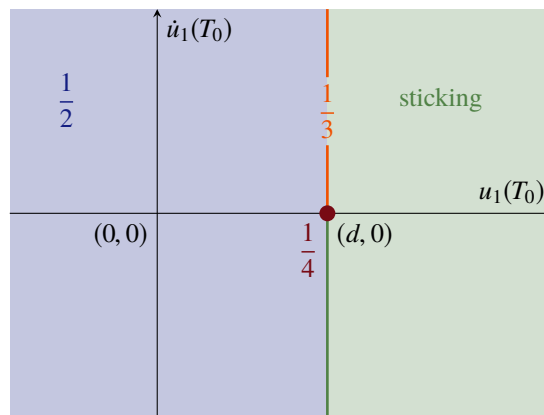
FIGURE 5. Power-root singularity ( 1/2 , 1/3 and 1/4 ) in the plane (u_1(T_0), \dot{u}_1(T_0)) which is isomorphic to the set \mathcal{H}^0 since u_2(T_0) = d and \dot{u}_2(T_0) = 0 . The blue area u_1 < d corresponds to grazing. The red branch u_1 = d and \dot{u}_1 > 0 corresponds to the beginning of a sticking phase. The green area u_1 > d corresponds to states within a sticking phase. The solid green line u_1 = d and \dot{u}_1 < 0 corresponds to the end of a sticking phase. The dark red dot correspond to a unique orbit the worst power-root singularity.
