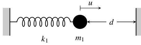
FIGURE 11. Simple unilaterally constrained one-dof system
