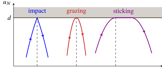
FIGURE 2. Possible types of contacts in discrete dynamics.
