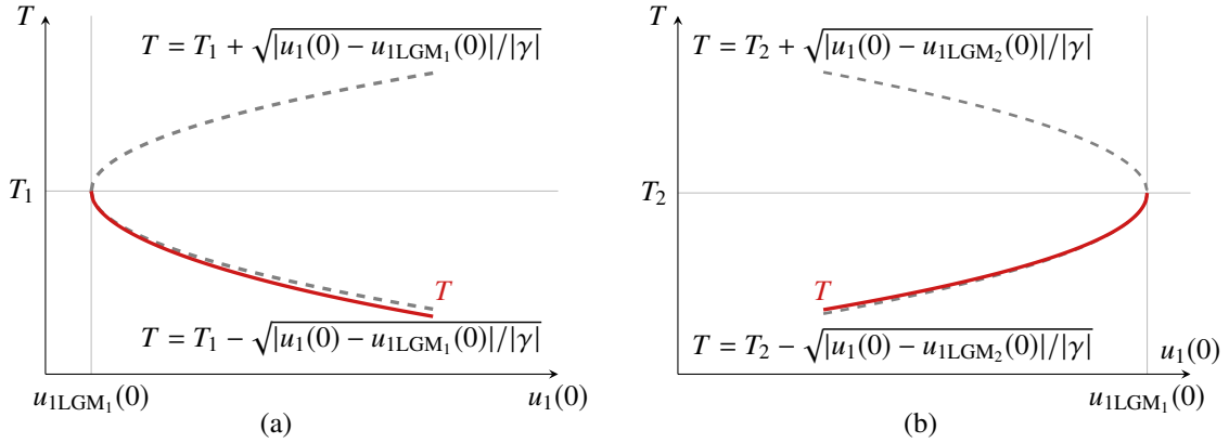
FIGURE 10. First Return Time (red lines) with respect to the initial displacement of the first mass: (a) near the first LGO, (b) near the second LGO.
