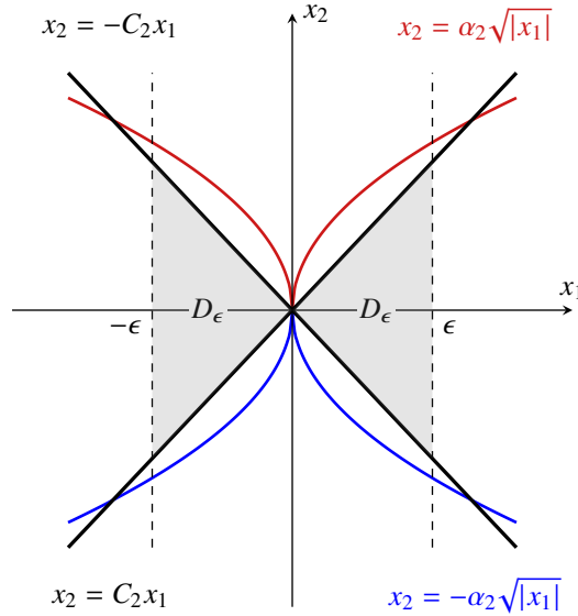
FIGURE 7. Neighborhood D_\epsilon
