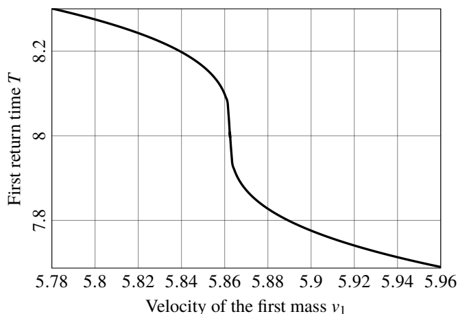
FIGURE 6. First Return Time T with respect to v_1 = \dot{u}_1 (near a periodic solution with one sticking phase per period [8]). A cubic-root singularity appears near v_1(0) = \dot{u}_1(0) = 5.86 .
