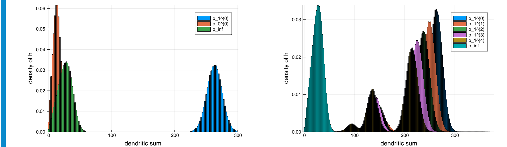
Fig: Distributions p_t^1 when f = 0.1 and parameters q_x^{+/-} = 0.5 . At time t = 0 , the two distributions are well separated (left) and then get closer (right).
