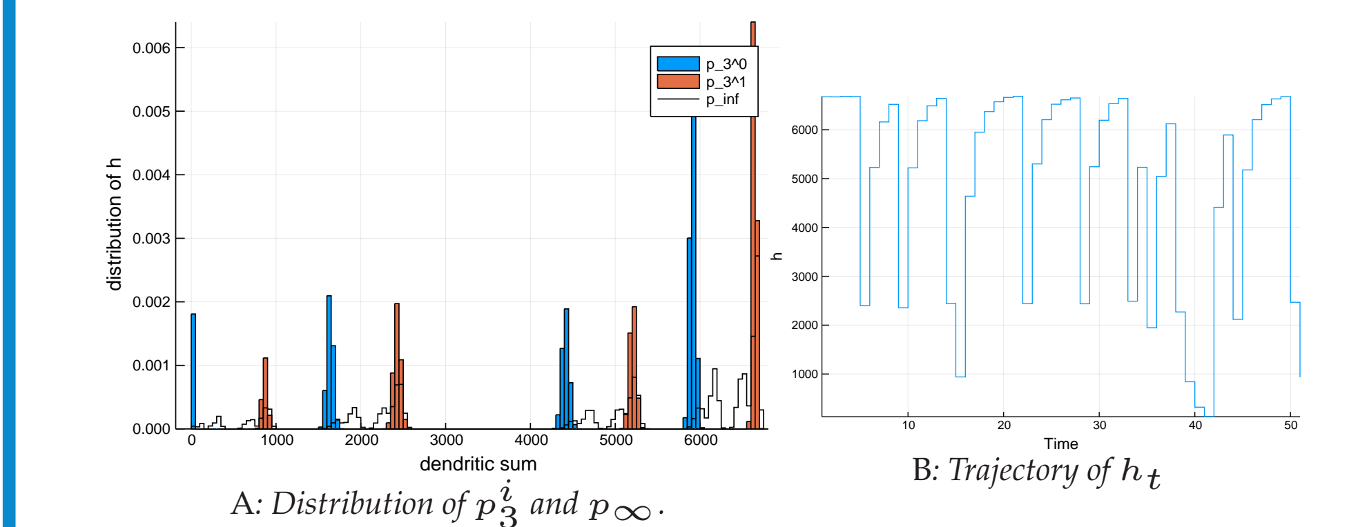
Fig: Parameters are the following: f = 0.5 , q^+ = 0.9 , q_{10}^- = 0.1 , q_{01}^- = 0.9
