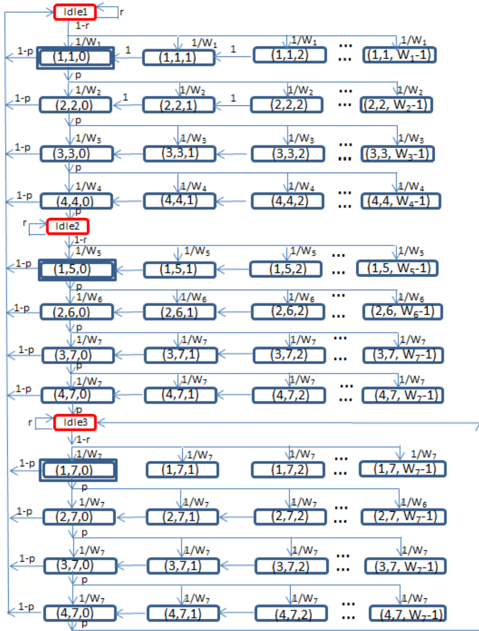
Fig. 2. The Markov chain of the collision avoidance method on shared slots with a backoff before each transmission.
