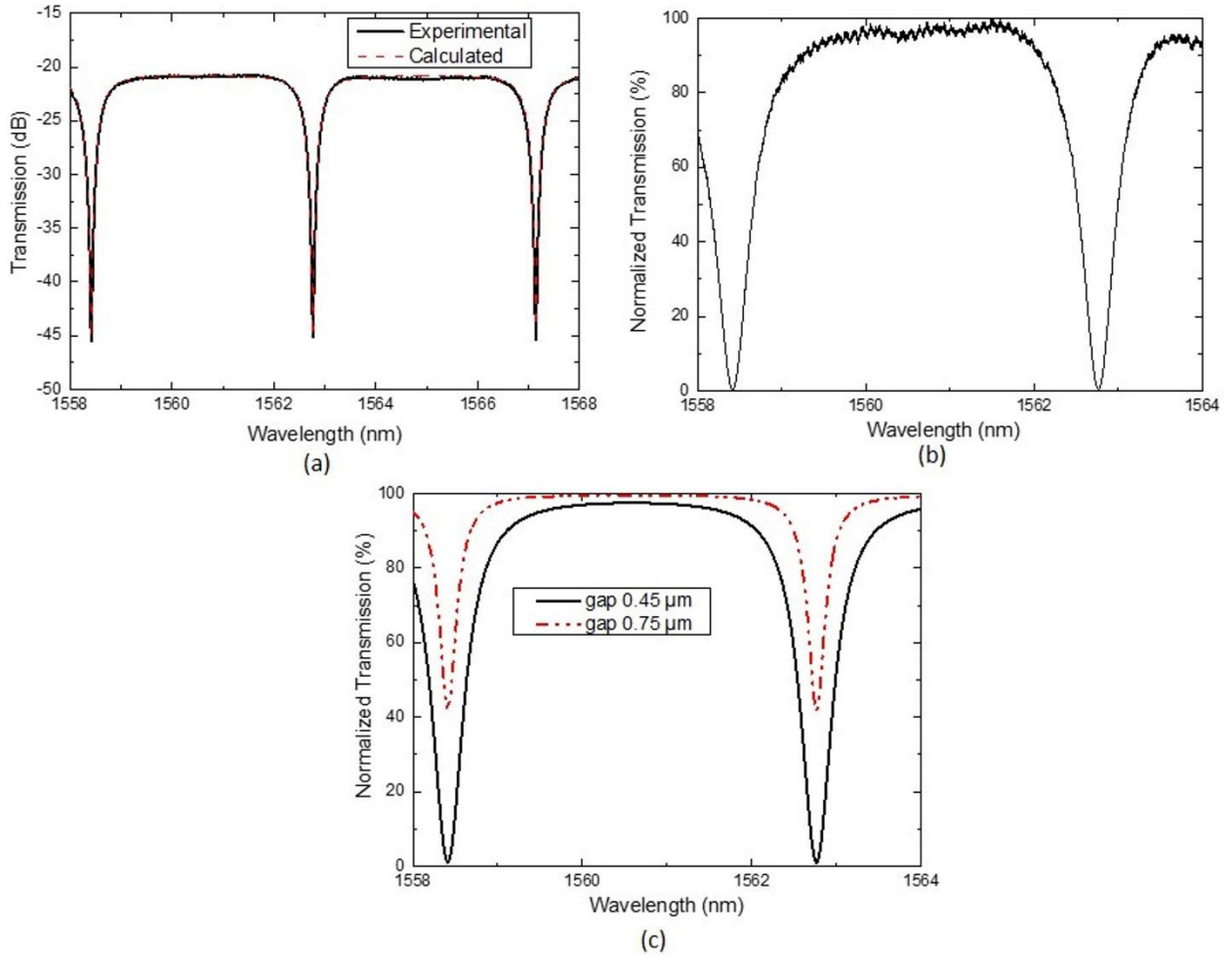
Figure 8 : Transmission spectra for one polarization of light of the porous silica racetrack MR : (a) Experimental and calculated spectra (gap of 0.45 \mu m), (b) normalized experimental spectrum (gap of 0.45 \mu m), (c) Calculated spectra for gaps of 0.45 \mu m and 0.75 \mu m.
