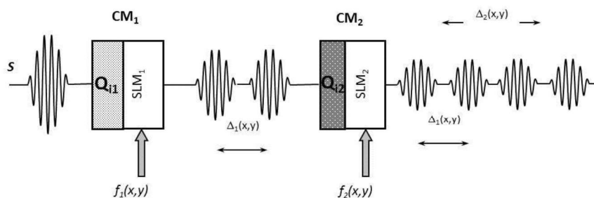
Fig.1. Schematic of the encryption setup
