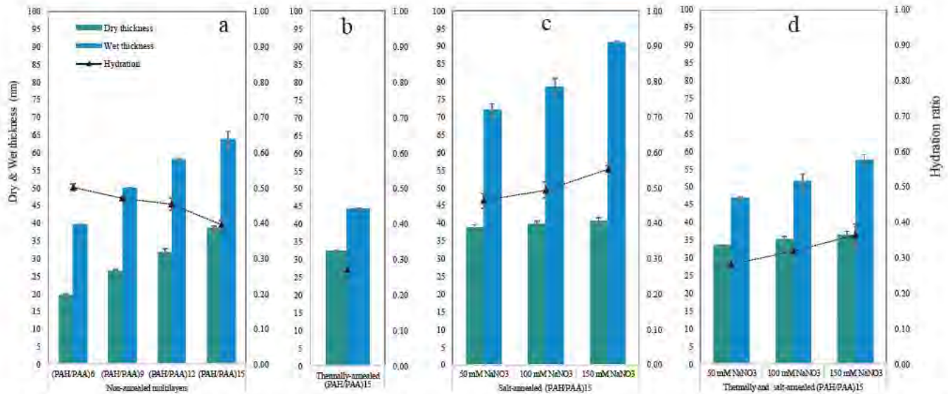
Fig. 1. Ellipsometric measurements of the coated silicon wafers of: (a) non-annealed, (b) thermally-annealed, (c) salt annealed and (d) thermally and salt-annealed PEMs.
