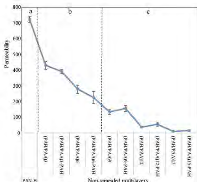
Fig. 2. Changes in the pure water permeability ( L m^{-2} h^{-1} bar^{-1} ) of the bare and coated membrane after deposition of (PAH/PAA) multilayers.
