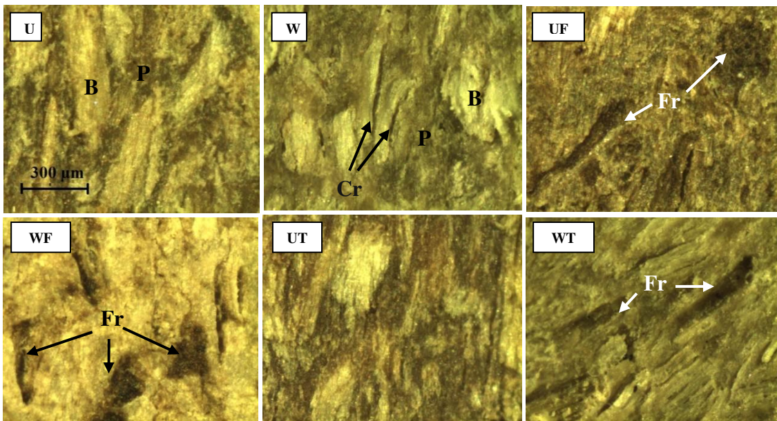
Fig. 3. Surface of control (non-pigmented) sample at different stages of degradation: U: un-weathered; W: weathered; F: after fungal attack ; T: after termite attack. B = bagasse fiber; P = Plastic; Cr = cracks; and Fr = fiber removal.
