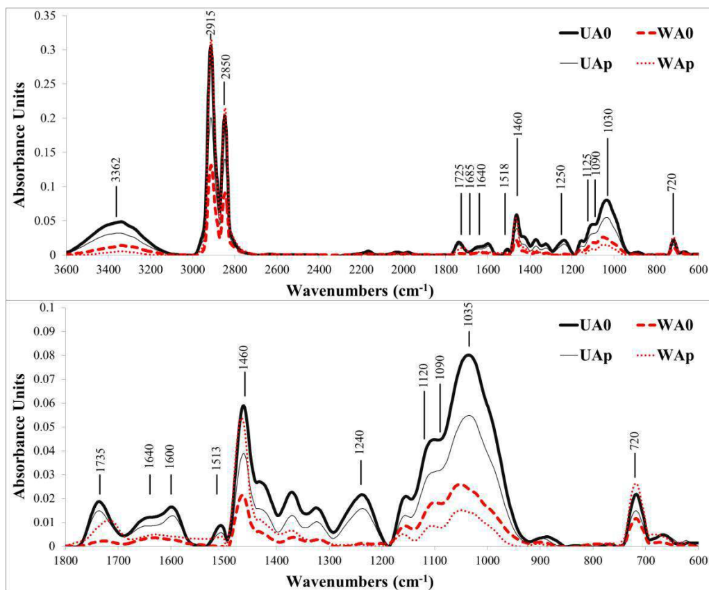
Fig. 1. ATR-FTIR spectra of control (A0) and pigmented sample (Ap) before (UA0, UAp) and after weathering (WA0, WAp)
