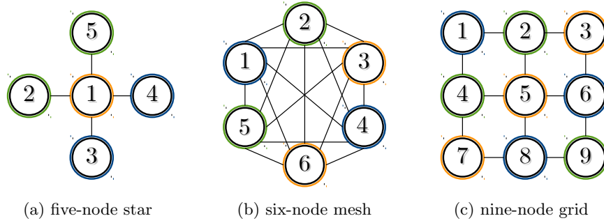
Figure C.16: Conflict graphs
