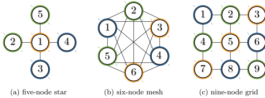
Figure C.16: Conflict graphs
