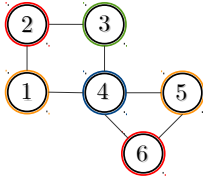
Figure 7: Conflict graph of the six-node network.
