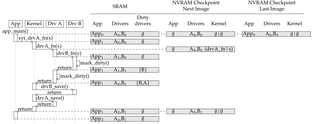
Fig. 10: Sequence diagram of a complex, i.e. , nested, system call with SRAM and NVRAM kernel data structures content.
