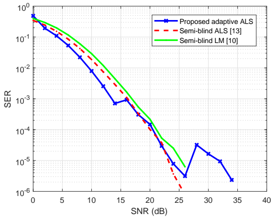
Fig. 2. SER versus SNR - Comparison between different receivers.
