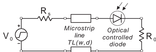
Figure 2. Equivalent schematic of atom-probe pulser.
