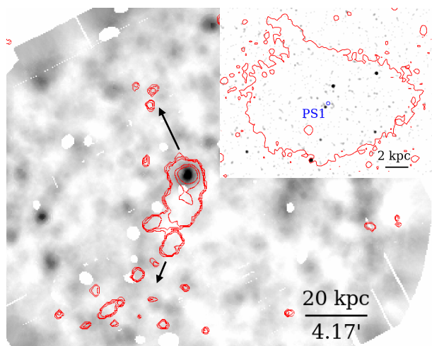
Fig. 5. The adaptively smoothed 0.4 - 1.3 keV XMM image of the NGC 4424 with the HI contours (from Chung et al. 2009) superposed. Bright X-ray point sources outside of the galaxy are masked. No soft X-ray enhancement is observed in the position of the HI tail. The two arrows at the north and at the south of the galaxy point towards the centre of Virgo cluster A and B, respectively. Their length is proportional to the distance to M87 and M49. The zoom-in region on the upper right shows the Chandra 0.5 - 7 keV image of the galaxy, with the H\alpha contours (as in Fig. 2) superposed. The small blue circle with a radius of 2'' shows the putative nuclear position, without a corresponding X-ray source. An obscured X-ray source 4.9'' to the southeast of the nucleus (PS1) is detected by Chandra .
