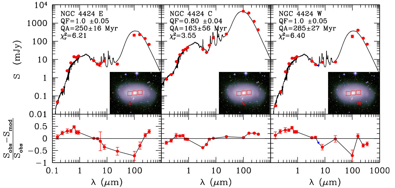
Fig. 11. The far UV-to-farIR SED of the three selected regions along the disc of NGC 4424 (from east to west). The observational data and their error bars are marked with a red filled dot, upper limits with a blue triangle. The black solid line shows the best fitted model. The inset shows the colour gri RGB image of the galaxy with overlaid the red boxes indicating the three fields used to study the SED with the CIGALE fitting code.
