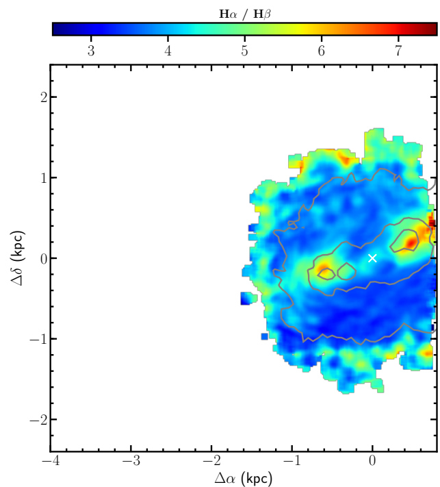
Fig. 6. The spaxel distribution of the Balmer decrement H\alpha/H\beta derived from the MUSE pixels with a signal-to-noise ratio S/N > 5 . The cross indicates the position of the nucleus, the grey contours the distribution of the H\alpha emitting gas (contour levels are \Sigma(H\alpha) = 5 \times 10^{-17} - 10^{-16} \text{erg s}^{-1} \text{cm}^{-2} \text{arcsec}^{-2} ).
