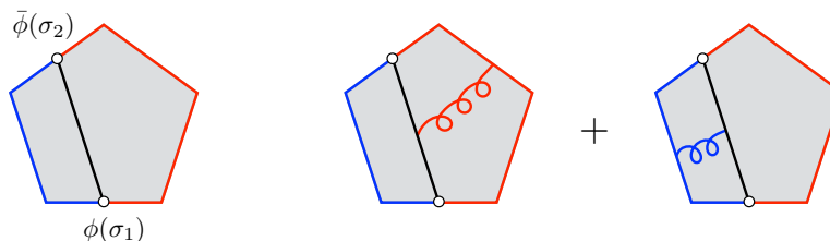
Figure 4. Tree level representation of the pentagon transition for matter fields, here taken to be scalars, and its first loop corrections. The two colors (red and blue) refer to the two gauge fields of the ABJM theory. Analyzing the first loop corrections could help understanding how to upgrade pentagon transitions to higher orders.
