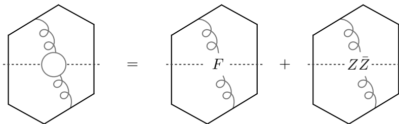
Figure 6. The OPE cut of the two loop contribution to the bosonic Wilson loop reveals a pair of matter fields, coming from the bubble correction to the Chern-Simons propagator. Its twist-1 component can take the form of a gluonic flux tube excitation F or of a spinon-anti-spinon pair Z\bar{Z} . They both start contributing at order O(g^2) at weak coupling, according to our pentagon conjectures.
