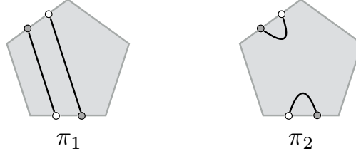
Figure 7. Cartoon of the matrix structure of the Z_A \bar{Z}^B \rightarrow Z_C \bar{Z}^D transitions. There are two structures for the two possible ways of contracting indices, \pi_1 \delta_A^C \delta_D^B + \pi_2 \delta_A^B \delta_D^C .
