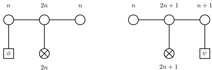
Figure 8. Dynkin diagrams encoding the matrix integral for descendants of a spinon Z \sim \phi and anti-spinon \bar{Z} \sim \psi . The top part is the Dynkin diagram for the SU(4) degrees of freedom with the labels indicating the numbers of corresponding auxiliary roots. They couple to the matter content represented by the bottom part. The small fermions are represented by the crossed nodes and the spinons by the boxes. The excitations numbers are chosen such that the overall charge matches the quantum number of \phi . We can view the small fermions as associated to a fermionic generator and extending the symmetry to OSp(4|2) .
