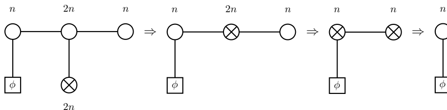
Figure 9. Integrating out the small fermions yields an effective matrix integral for a new system with the matrix structure depicted here. One can keep going until one is left with a single node coupled to the spinon. The structure of the latter node is akin to the one for an SL(2) spin chain. The manipulations carried out here are reminiscent of the dualization procedure for super spin chains.
