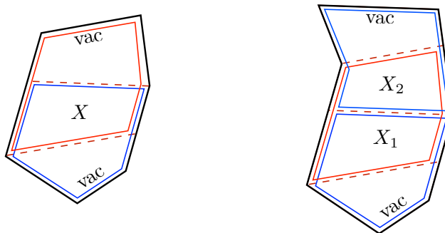
Figure 5. Decomposition of hexagon and heptagon Wilson loops into overlapping sequences of pentagons. For the hexagon, we have two pentagons overlapping on one square and correspondingly only one complete sum over intermediate states is needed. The heptagon has an extra hat, one more pentagon and middle square, and two sums are needed.
