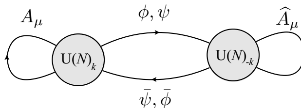
Figure 1. Quiver diagram for the ABJM theory.
