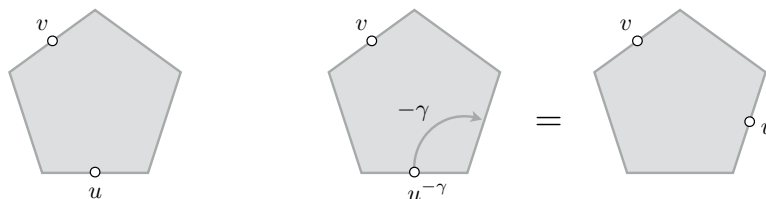
Figure 3. Left panel: cartoon for pentagon transition P(u|v) between a flux tube excitation smeared with rapidity u at the bottom and one with a rapidity v at the top. Right panel: under the inverse mirror rotation -\gamma : u \rightarrow u^{-\gamma} an excitation is moved anticlockwise to the neighbouring edge. The result is a pentagon transition with bottom and top being exchanged, P(u^{-\gamma}|v) = P(v|u) .
