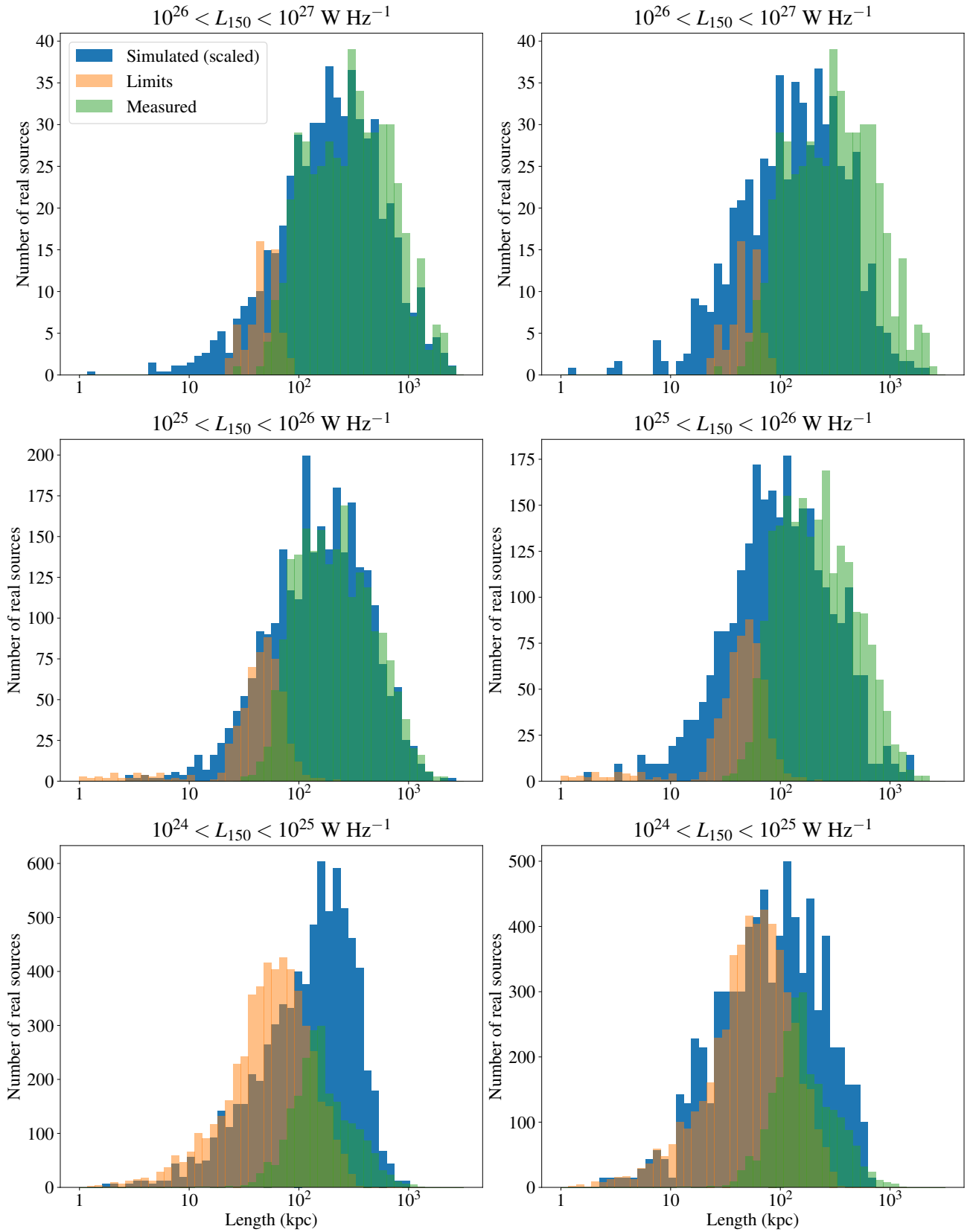
Fig. A.1. Distributions of real and simulated projected sizes for three luminosity ranges (from top to bottom panels, three slices of the P – D diagram of Fig. 8) and two lifetime distributions (left panels: model (i), uniform, right panels: model (ii), log-uniform).
