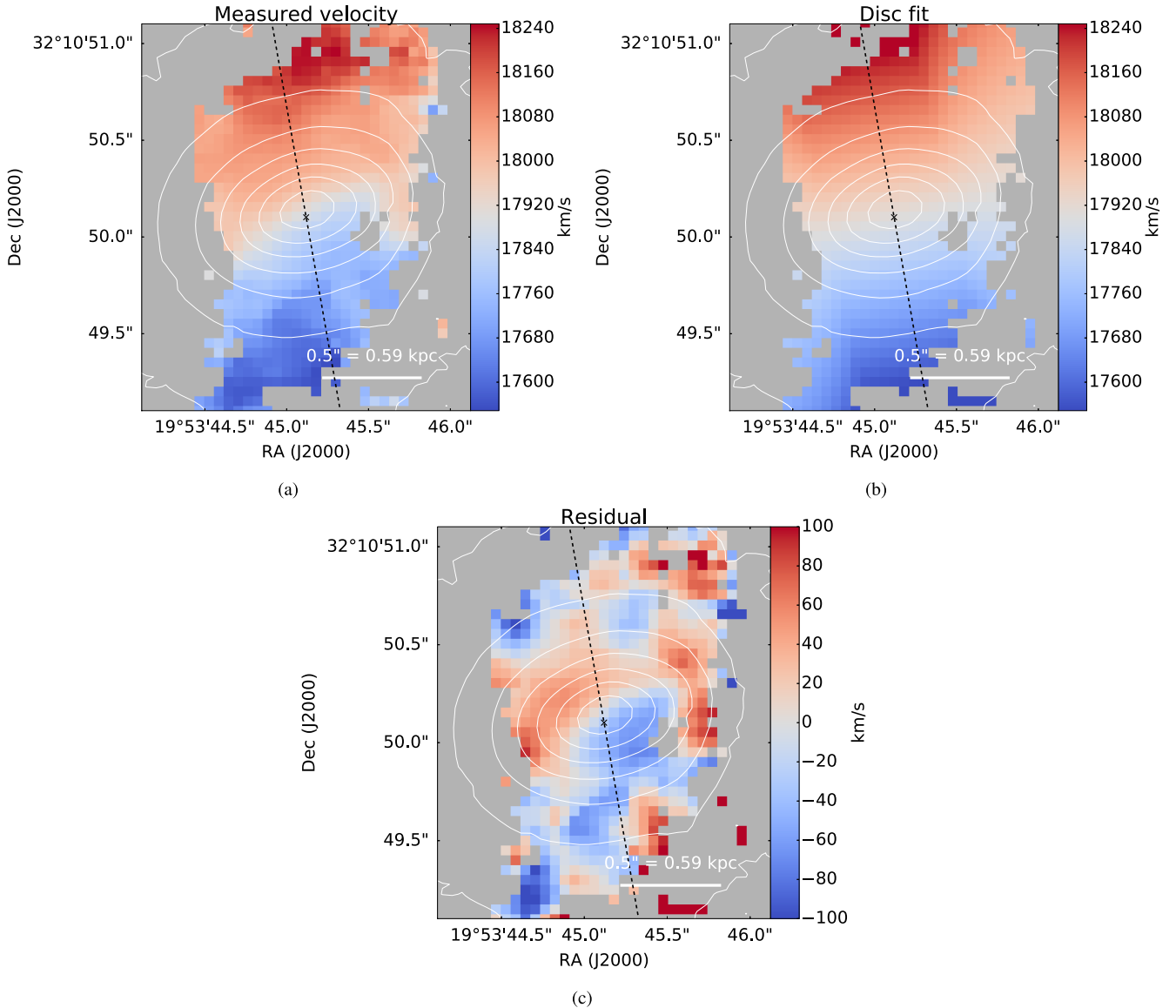
Figure 4. Kinematics of the H 2 1–0 S(1) emission line; (a): measured radial velocity, (b) radial velocity of the model fit, and (c) the residual. With the exception of the residual plot, all velocities are given with respect to the local standard of rest. The cross represents the location of the nucleus (i.e. the peak in the K -band continuum). Fig. 5 shows a cross-section of the radial velocities taken along the dashed black line.
