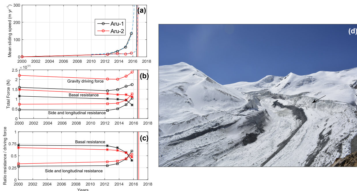
Figure 9. (a) Mean sliding speed of the detachment zone for Aru-1 (black) and Aru-2 (red) glaciers. The dashed blue lines show predicted speed following an empirical law of slope failure (Voight, 1990). (b) Force balance acting on the detachment of Aru-1 (black) and Aru-2 (red). (c) Ratio of resisting force over driving force for Aru-1 (black) and Aru-2 (red). Vertical lines show collapse dates in the three panels. (d) The Aru-2 glacier detachment zone on 4 October 2016 (Picture from T. Yao). The side resistance computed in the force balance analysis arises from lateral shearing on the right side of the detachment (black arrow).
