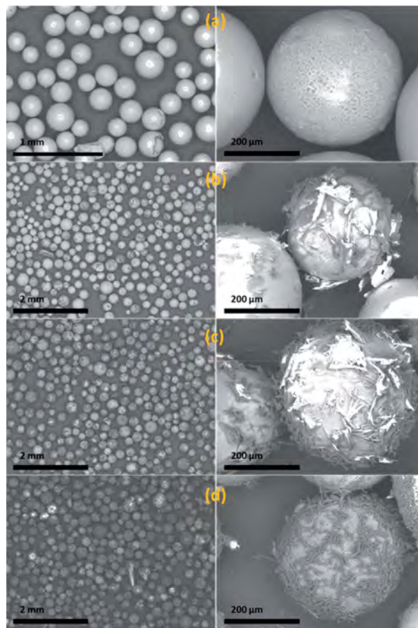
Figure 2. SEM images of (a) native SS particles and HQ-SS composite material with an HQ content of (b) 0.41 \pm 0.01 , (c) 0.27 \pm 0.04 , and (d) 0.10 \pm 0.02 \text{g}^{\text{HQ}}/\text{g}^{\text{Support}} .
