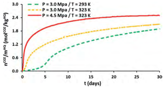
Figure 3. Molar quantity of gas captured by enclathration as a function of time using powdered HQ normalized by mass of HQ. Experiments with CO 2 at (green line) 293 K/3.0 MPa, (yellow line) 323 K/3.0 MPa, and (red line) 323 K/4.5 MPa.
