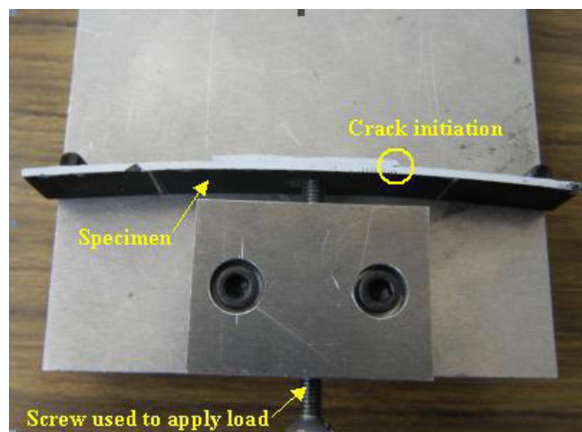
Fig. 3: Three-point-bending rig with specimen in place
