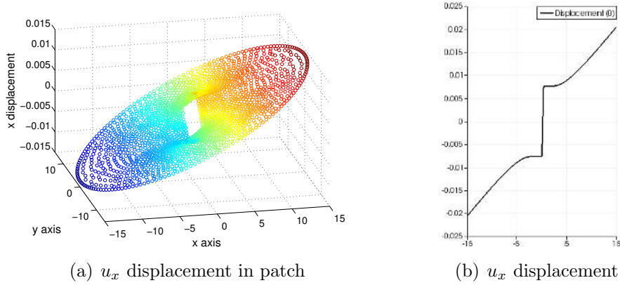
Figure 2: displacement in circular patch for depth d = 3 crack in displacement database
