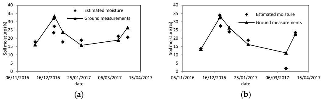
Figure 5. Temporal variations of the remotely sensed and measured soil moisture, for two reference fields: (a) Field P19; (b) Field P21.
