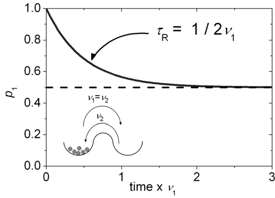
FIG. 4. Evolution of the probability p_1 to find a nanoparticle in the initially full potential well as a function of t \times \nu_1 . The result is an exponential decay function with a time constant of 1/2\nu_1 . (Inset) Illustration of the emptying of an initially full potential well through a reversible jump over the barrier.
