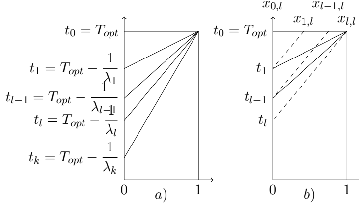
Figure 2: The definition of t_l is given in a) and the definition of x_{i,l} is given in b) where dashed lines have the same slope for constant \Sigma .
