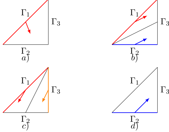
Figure 1: The characteristic vectors of K_{ij} in the case \Sigma is constant: a) in the case a_{ij}/b_{ij} < 0 ( 1 \leq i \leq k < k+1 \leq j \leq k+m or 1 \leq j \leq k < k+1 \leq i \leq k+m ), b) in the case 0 < a_{ij}/b_{ij} < 1 ( 1 \leq i < j \leq k or k+1 \leq j < i \leq k+m ), c) in the case a_{ij}/b_{ij} > 1 ( 1 \leq j < i \leq k or k+1 \leq i < j \leq k+m ), and d) in the case a_{ij}/b_{ij} = 1 ( 1 \leq i = j \leq k+m ).
