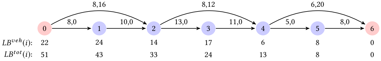
Figure 6 Lower bounds for the graph of Figure 4.
