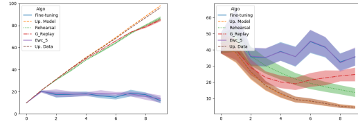
(g) Fitting Capacity CVAE
