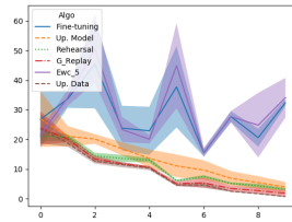
(f) FID WGAN
