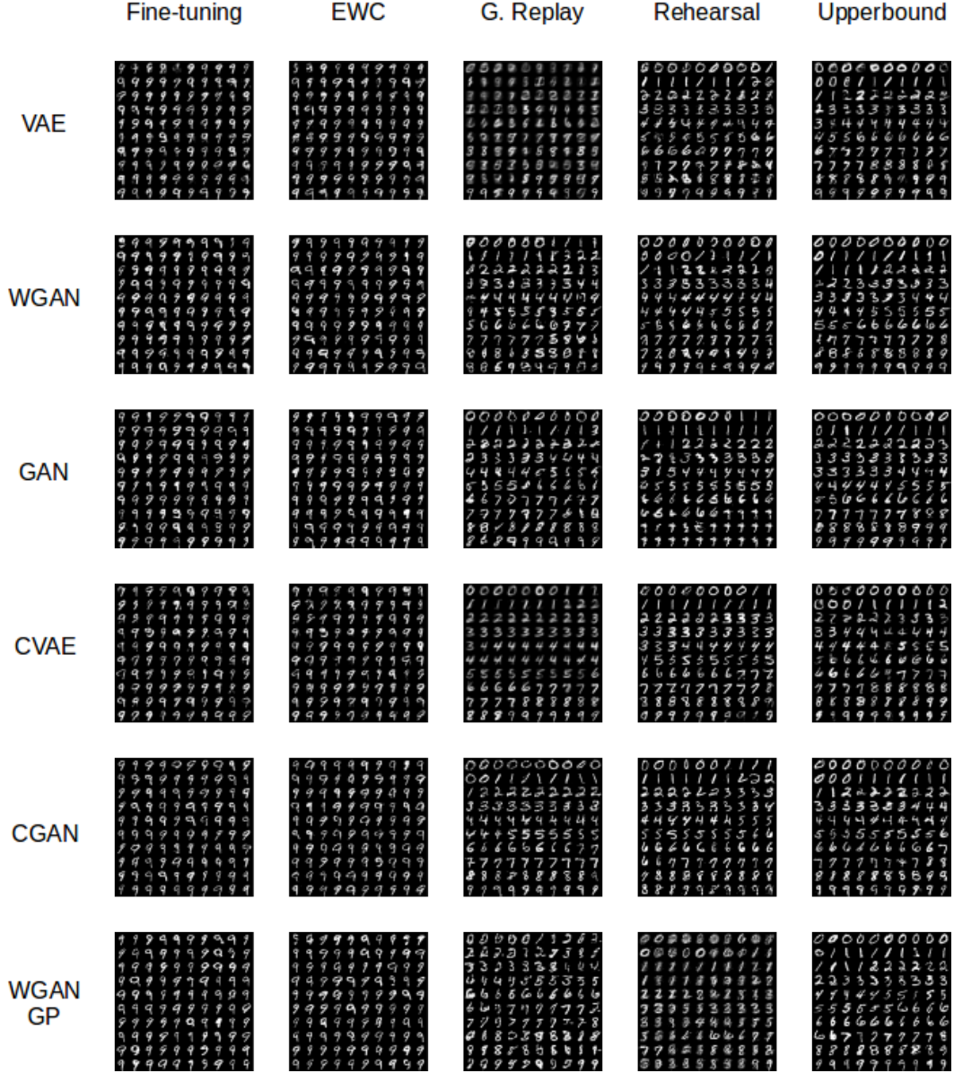
Figure 13: MNIST samples for each generative model and each Continual Learning strategy, at the end of training on 10 sequential tasks. The goal is to produce samples from all categories.
