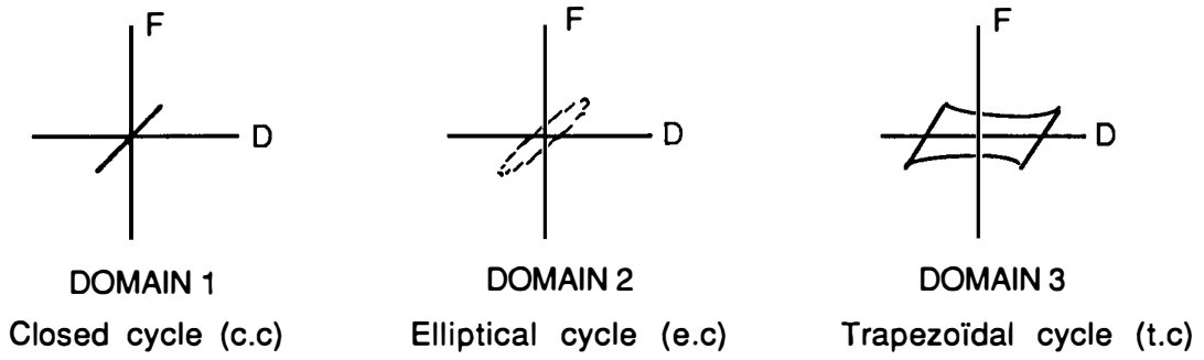
Figure 3 : Characteristic friction loops
