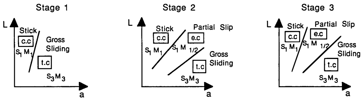
Running Condition Fretting Maps (L : Load, a : Amplitude)
