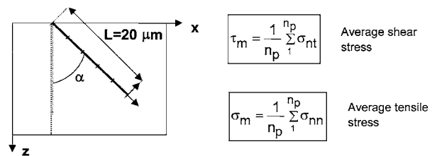
Fig. 3. Theoretical approach to crack analysis within the contact meridian plane.
