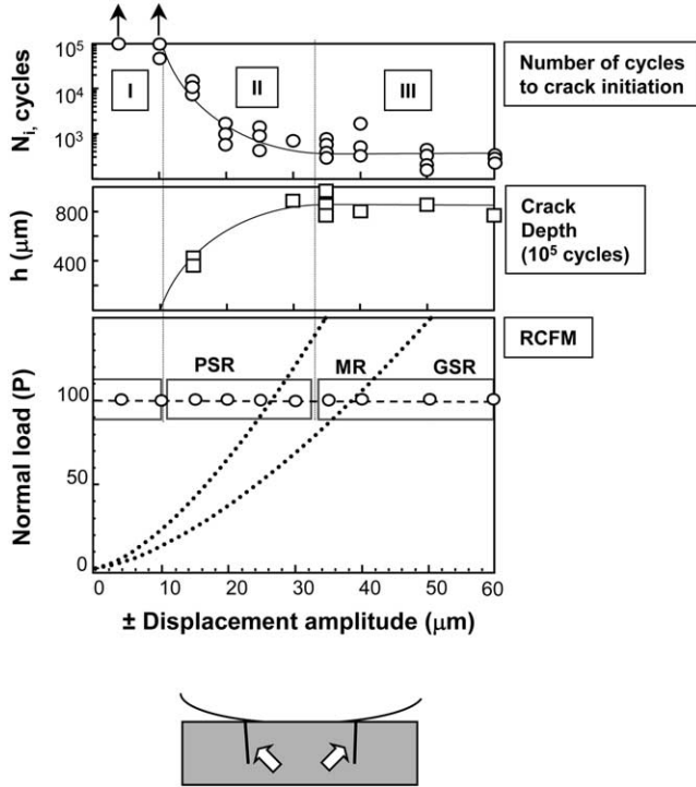
Fig. 8. Number of cycles to crack initiation, N_i , and crack depths, h , within the various regimes of the RCFM under a fretting wear loading (see text for comments on regions I, II and III).
