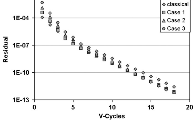
Fig. 10. Residual with three refinement strategies.
