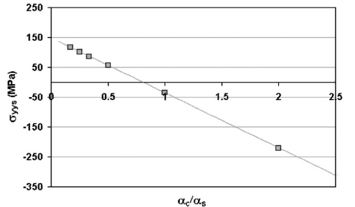
Fig. 11. \sigma_{yy} peak stresses at the surface as a function of \alpha_c/\alpha_s , H_c = 10 \mu\text{m} .
