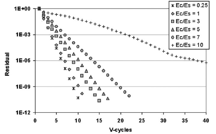
Fig. 8. Residual on finest level as a function of E_c/E_s ratio with H_c = 0.5 mm.
