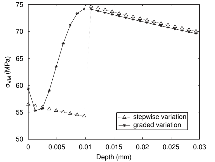
Fig. 15. \sigma_{vm} in the center of the solid, H_c = 10 \mu\text{m} .
