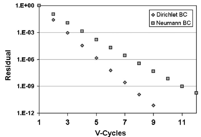
Fig. 3. Residual on finest level for Dirichlet and Neumann BC.
