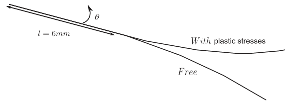
Fig. 23. Crack propagation path with and without plastic stresses ( l = 6 \text{ mm} , \theta = 15^\circ , \mu_{\text{crack}} = 0.5 , \mu_{\text{wheel-rail}} = 0.025 ).
