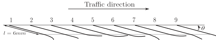
Fig. 28. Crack path after 5 propagation steps for a network of 9 parallel cracks \theta ( l = 6 mm, \theta = 15^\circ , \mu_{crack} = 0.5 , \mu_{wheel-rail} = 0.1 ).
