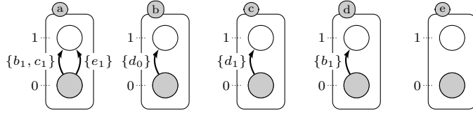
Figure 1: An example of ABAN
