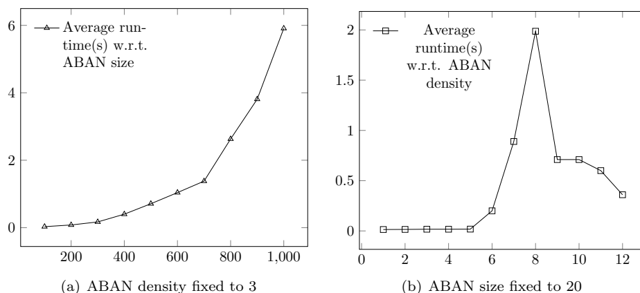
Figure 9: Runtime of ASPReach on random ABANs
