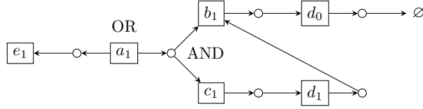
Figure 2: Visualization of LCG, with the squares representing local states and small circles representing solution nodes. \emptyset signifies that there is no need to link any transitions, i.e the former state d_0 is in the initial state.
