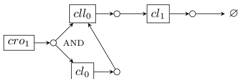
Figure 7: One LCG in \lambda -phage model, automaton cl appears in both branches of the AND gate. Static analyzer Pint cannot decide whether in this case cro_1 is reachable or not, because it does not consider the order in the state sequence even though there exists a solution is of length 3: cll_0 :: cl_0 :: cro_1 corresponding to the trajectory \{cl_1\} \rightarrow cl_{ll_0} :: \{cl_{ll_0}\} \rightarrow cl_0 :: \{cl_{ll_0}, cl_0\} \rightarrow cro_1 .
