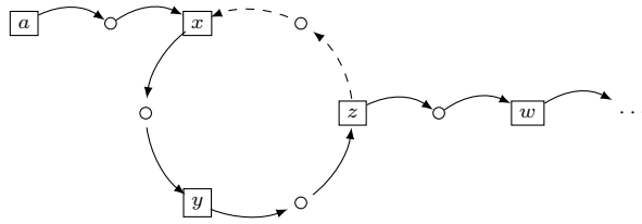
Figure 4: LCG l containing cycle x \rightarrow \circ \rightarrow y \rightarrow \circ \rightarrow z \rightarrow \circ \rightarrow x
