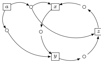
Figure 5: x, y, z all have external links, thus none of the links can be discarded
