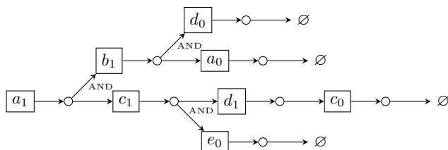
Figure 8: This counterexample shows former PermReach is inconclusive if multiple states of one automaton appear in the branches of one AND gate ( d_0 and d_1 in this example). However there exists a consistent state sequence: d_1 :: b_1 :: c_1 :: a_1 corresponding to the trajectory \{c_0\} \rightarrow d_1 :: \{d_0, a_0\} \rightarrow b_1 :: \{d_1, e_0\} \rightarrow c_1 :: \{b_1, c_1\} \rightarrow a_1 which could be found by ASPReach.
