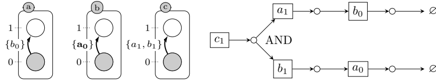
Figure 3: \Sigma = \{a, b, c\} , T = \{\{b_0\} \rightarrow a_1, \{a_0\} \rightarrow b_1, \{a_1, b_1\} \rightarrow c_1\} , \omega = c_1
