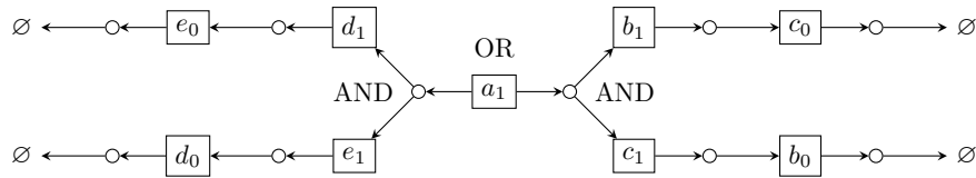
Figure 6: If an LCG contains such structure, the result could be inconclusive. However the inconclusiveness requires a_1 does not possess other reachable branches.
