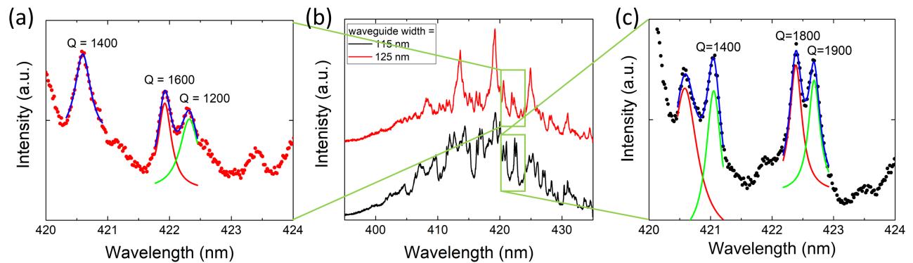
FIG. S6. Loaded Q factor of two devices with a disk diameter of 3\ \mu\text{m} , a waveguide bending angle of 90^\circ , a gap of 90 nm, and waveguide widths of 115 to 125 nm. a) Zoom-in of the w = 125\ \text{nm} curve and Lorentzian fits giving loaded Q factors of 1200 to 1600. b) Full spectra of both devices. c) Zoom-in of the w = 115\ \text{nm} curve and Lorentzian fits giving loaded Q factors of 1400 to 1900.
