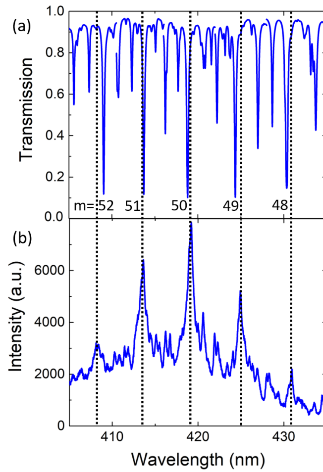
FIG. S2. Comparison of a) simulation and b) measurement for a 3 \mu\text{m} diameter disk. The mode positions match well and the azimuthal numbers of the first order radial modes is clearly identified.
