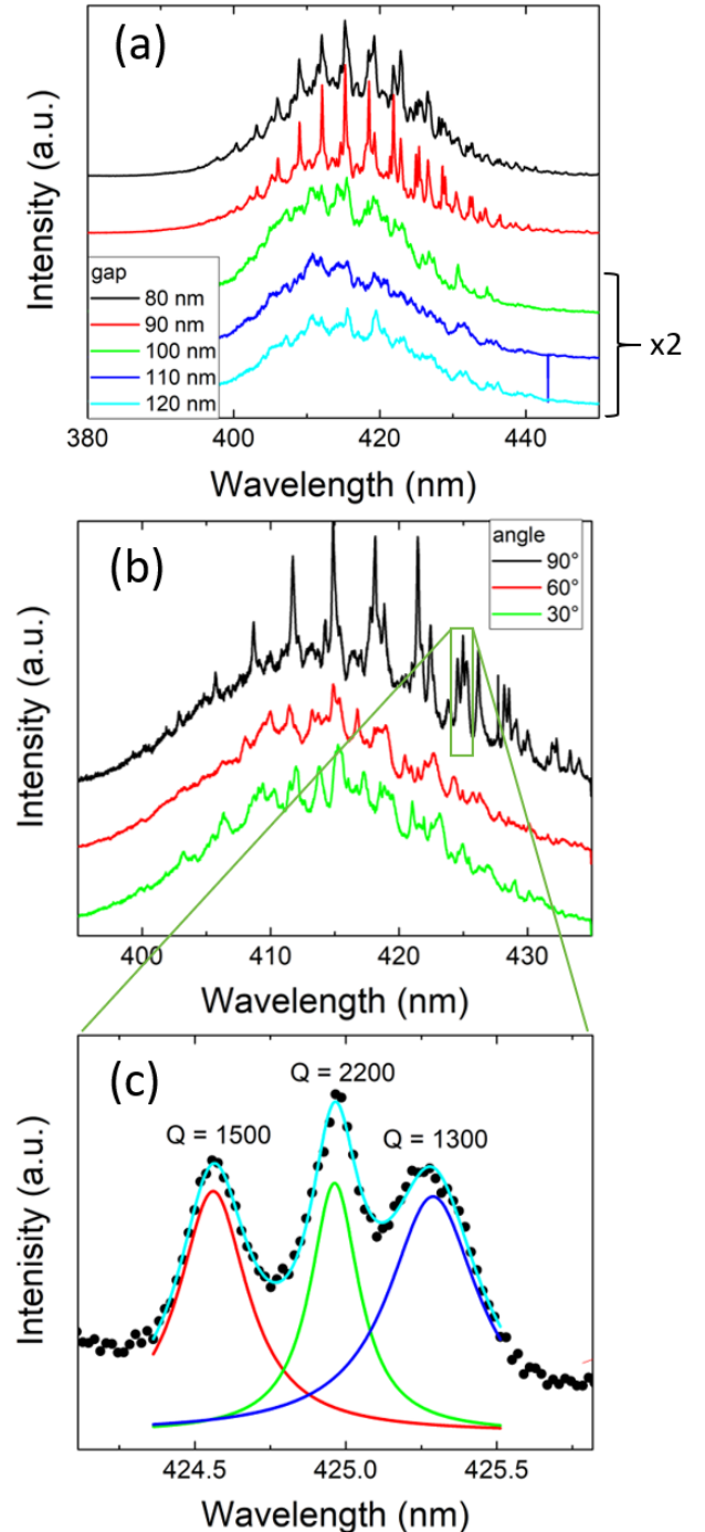
FIG. 3. PL measurements integrated over one grating coupler on the CCD for devices with a disk diameter of 5 \mu\text{m} , a waveguide width of 155 nm and a grating period of 210 nm. a) The waveguide bending angle is 90° and the gap sizes vary between 80 nm and 120 nm. The spectra for g = 100 - 120 nm have been multiplied by 2 for better visibility of the modes. b) The gap is 90 nm and the bending angle has been varied between 90° and 30°. c) Close-up of three modes of the 90° spectrum in b) showing Lorentzian fits and the corresponding Q factors.
