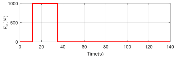
Fig. 2. Lateral wind gust input F_w .
