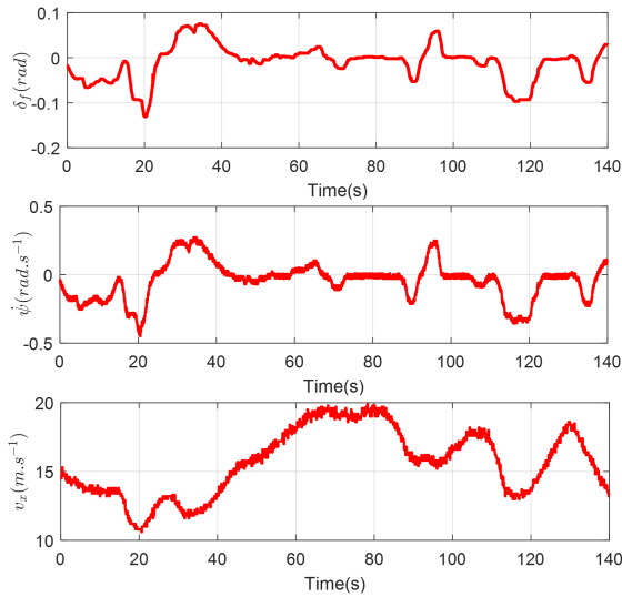
Fig. 3. Steering angle \delta_f , yaw rate \dot{\psi} and longitudinal velocity v_x .
