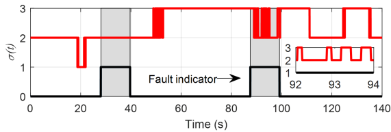
Fig. 4. Switching law and faults zone.
