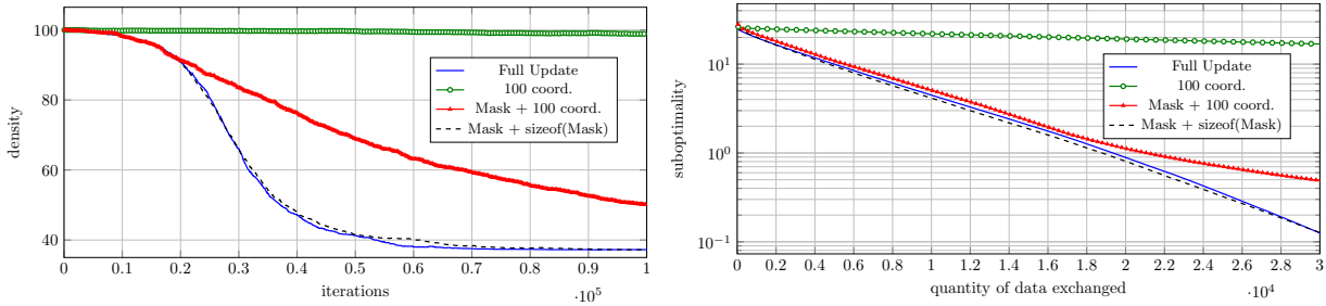
Figure 3: Performance of the algorithms on the logistic regression problem with the epsilon dataset: identification properties (at the left) and convergence with respect to communication cost (at the right).
