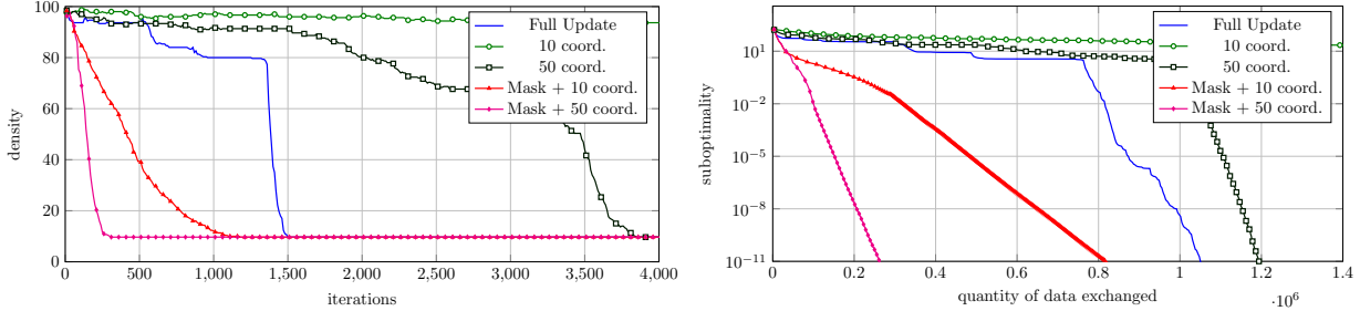
Figure 1: Performance of the algorithms on the synthetic lasso problem: identification properties (at the left) and convergence with respect to communication cost (at the right).
