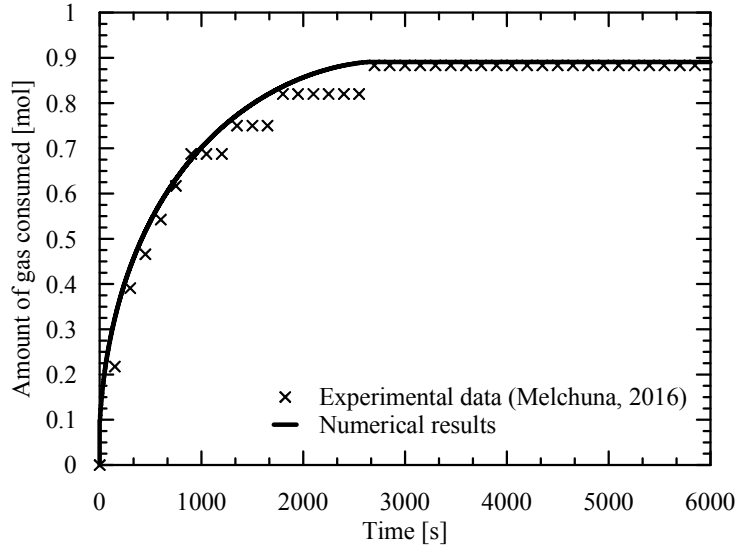
Figure 2. Comparison of model results against experimental data of Melchuna et al. [20] for the amount of gas consumed over time due to hydrate formation.
