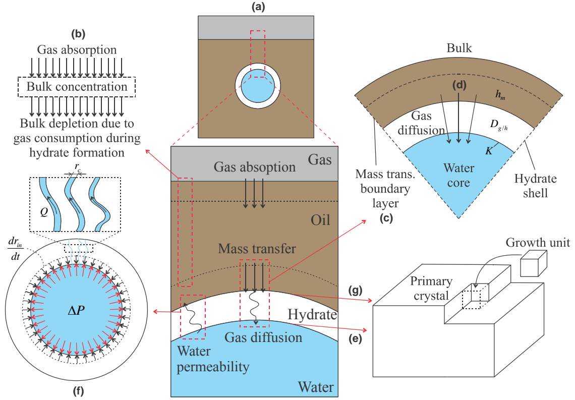
Figure 1. (a) Gas hydrate shell formed around a water droplet in oil continuous phase, which is in contact with the gas free phase. (b) Gas absorption by the bulk competes with gas consumption due to hydrate formation. (c) Gas consumption due to hydrate formation creates a concentration boundary layer around the particle. (d) Gas diffuses through the hydrate shell. (e) Once the gas reaches the inner surface, crystal integration process takes place, causing inner growth. (f) Core-shrinkage makes water to be expelled through the porous hydrate shell. (g) Once water reaches the outer surface, crystal integration process happens with consequent outer growth.
