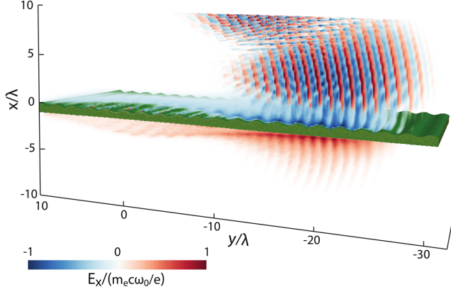
FIG. 4. 3D particle-in-cell simulation snapshot of laser-grating interaction, showing the electric field component E_x and an isosurface highlighting the target at time t = 35\lambda/c after the beginning of the interaction. Only the z < 0 region of the simulation box is shown in order to highlight the field distribution. In the upper part of the picture, the distribution of E_x is related to the diffracted pulse, while that in the lower part corresponds to a surface plasmon propagating in the -\hat{y} direction.
