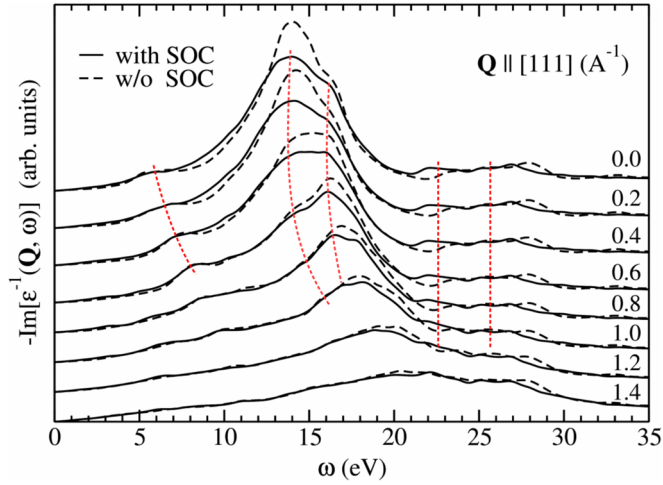
FIG. 5. EEL spectra with (solid lines) and without (dashed lines) SOC of bulk Bi at various values of \mathbf{Q} along the [111] direction in framework of the reciprocal basis vectors of BZ ( \text{\AA}^{-1} ). Curves have been shifted vertically for clarity. Calculations have been performed within TDDFpT using the LDA XC functional. Red dashed lines are guides for the eye showing the dispersion of the peaks.
