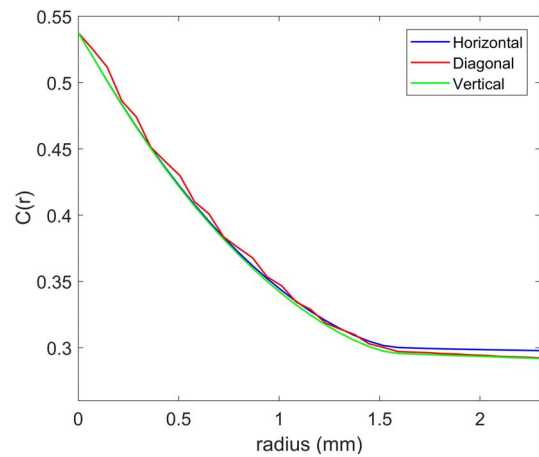
Fig. 9. Mean covariance on 100 silhouette images of the population of PMMA spheres in the three main directions.
