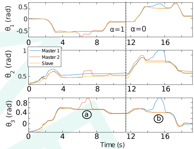
Figure 7: Angular positions for the trajectory performed in free motion
