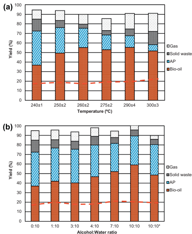
Fig. 2. The effects of the temperature (a) and the addition of co-solvent (b) on the products distribution. Note: The red dashed line indicates the light fraction in bio-oil. In Fig. 2b, 10:10* represents the results obtained using methanol. (For interpretation of the references to colour in this figure legend, the reader is referred to the web version of this article.)
