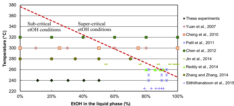
Fig. 1. Summary of the operating conditions applied by several authors using microalgae and other substrates. Note: The dashed line separates the sub-critical and super-critical conditions in ethanol:water mixtures (Yuan et al., 2007). In green, experiments carried out with microalgae and ethanol:water mixtures. In blue, microalgae and methanol:water mixtures. In red, other substrates and ethanol:water mixtures.
