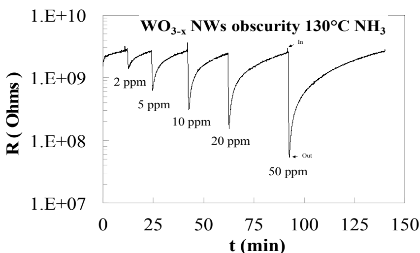
Figure 2. Resistance variation of WO_{3-x} NWs with NH_3 exposure with the concentrations of 2, 5, 10, 20 and 50 ppm at a working temperature equals to 130 °C.
