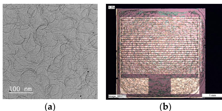
Figure 1. (a) TEM image of WO_{3-x} NWs and (b) Si-SiO 2 substrate picture with WO_{3-x} NWs dropped on it.
